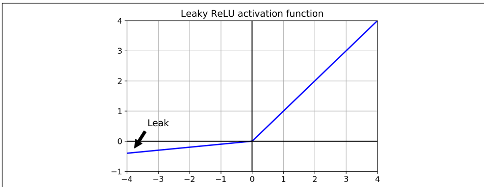
Figure 11-2. Leaky ReLU
