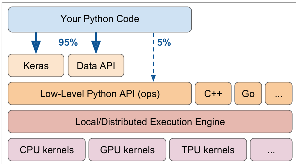
Figure 12-2. TensorFlow's architecture
