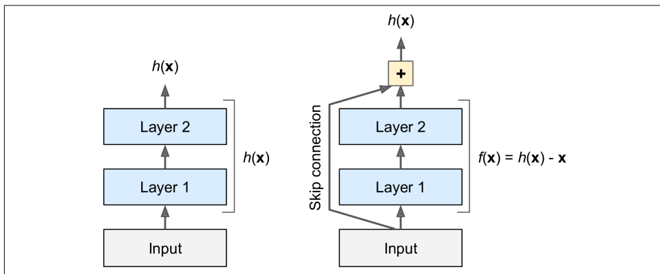
Figure 14-15. Residual learning
