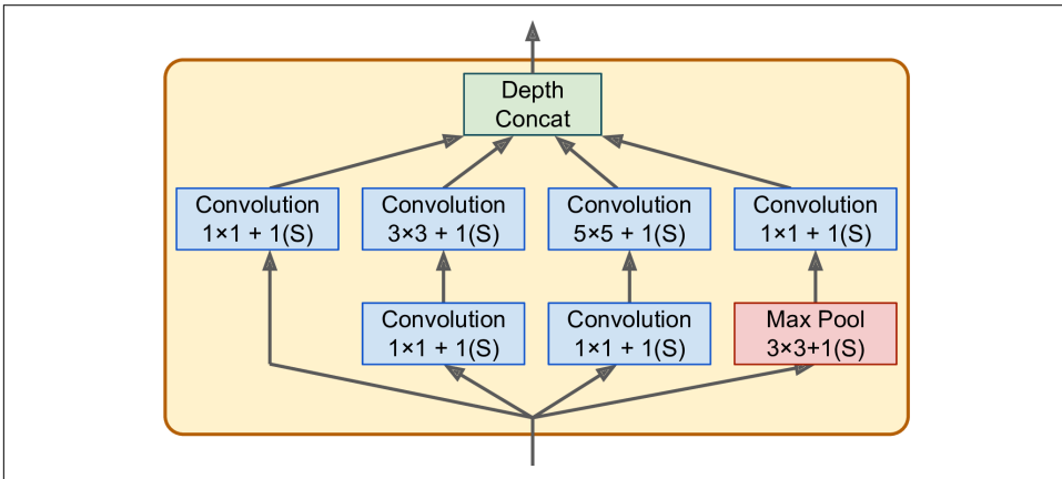
Figure 14-13. Inception module
